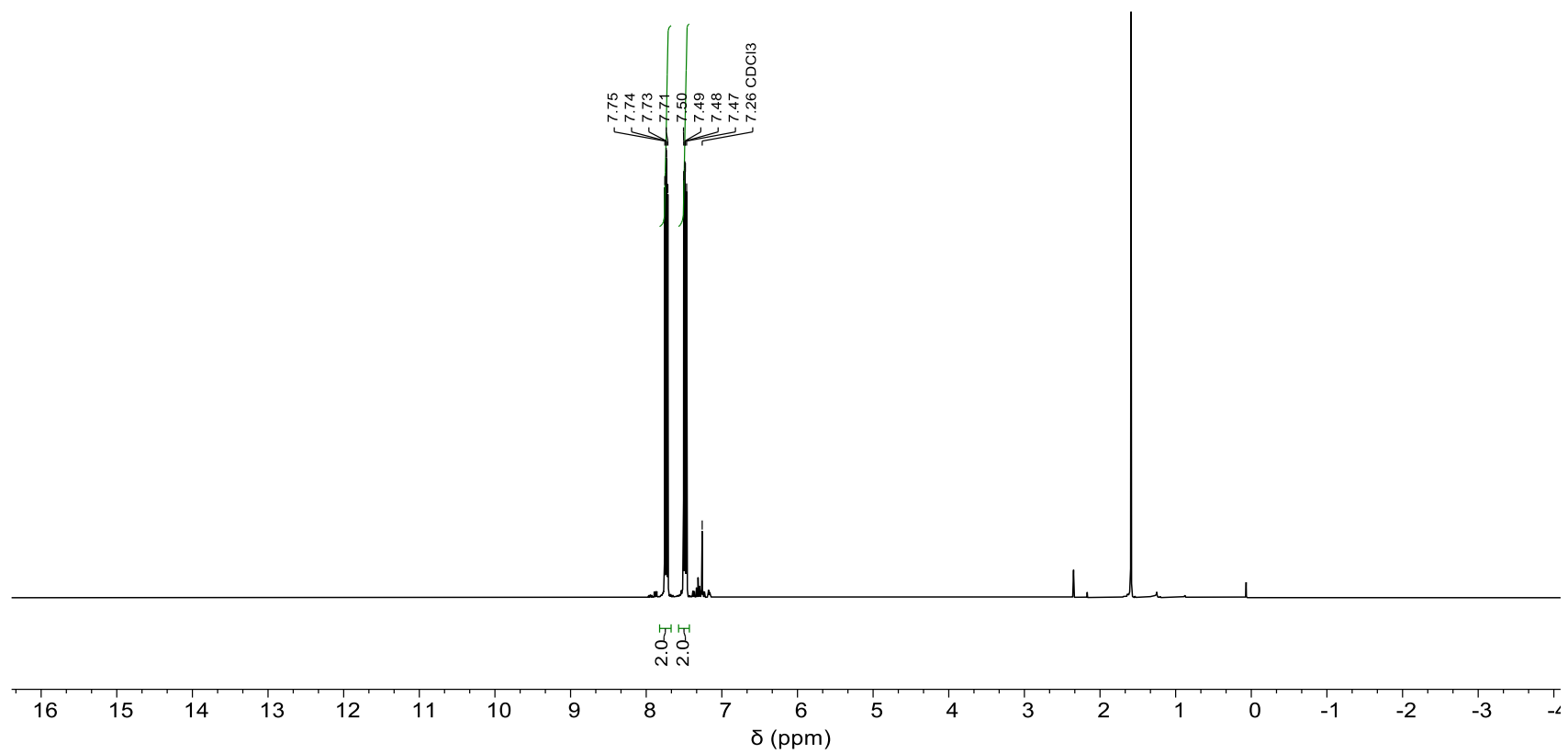
1 H NMR (400 MHz, CDCl 3 ) of 2,3,7,8-tetrafluorothianthrene-S-oxide (2).
